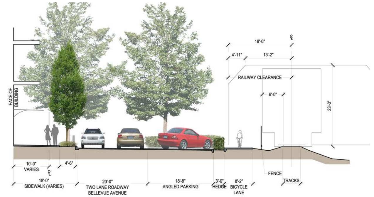
D SECTION AT BELLEVUE AVE. 1/16" = 1'-0"
