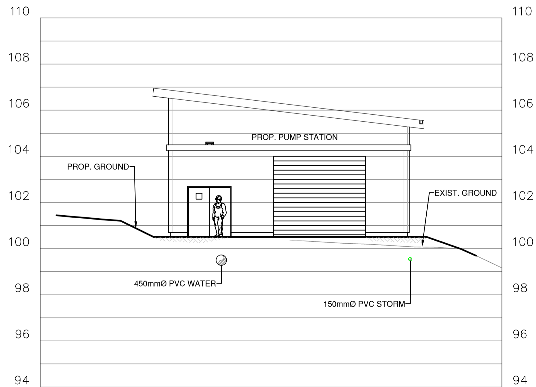
2 SECTION C101 1:100
